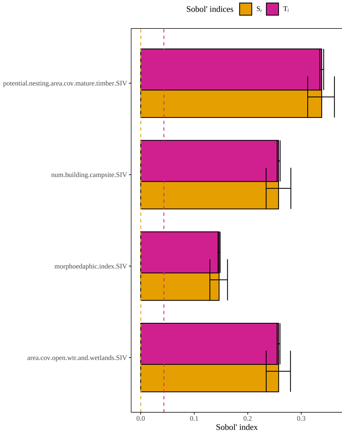
Figure 4. Results of a sensitivity analysis for the baldeagleBreeding model based on an arithmetic mean structure. Dashed lines represent baseline numerical approximation error for S_i and T_i ( i.e. , dummy variables).
