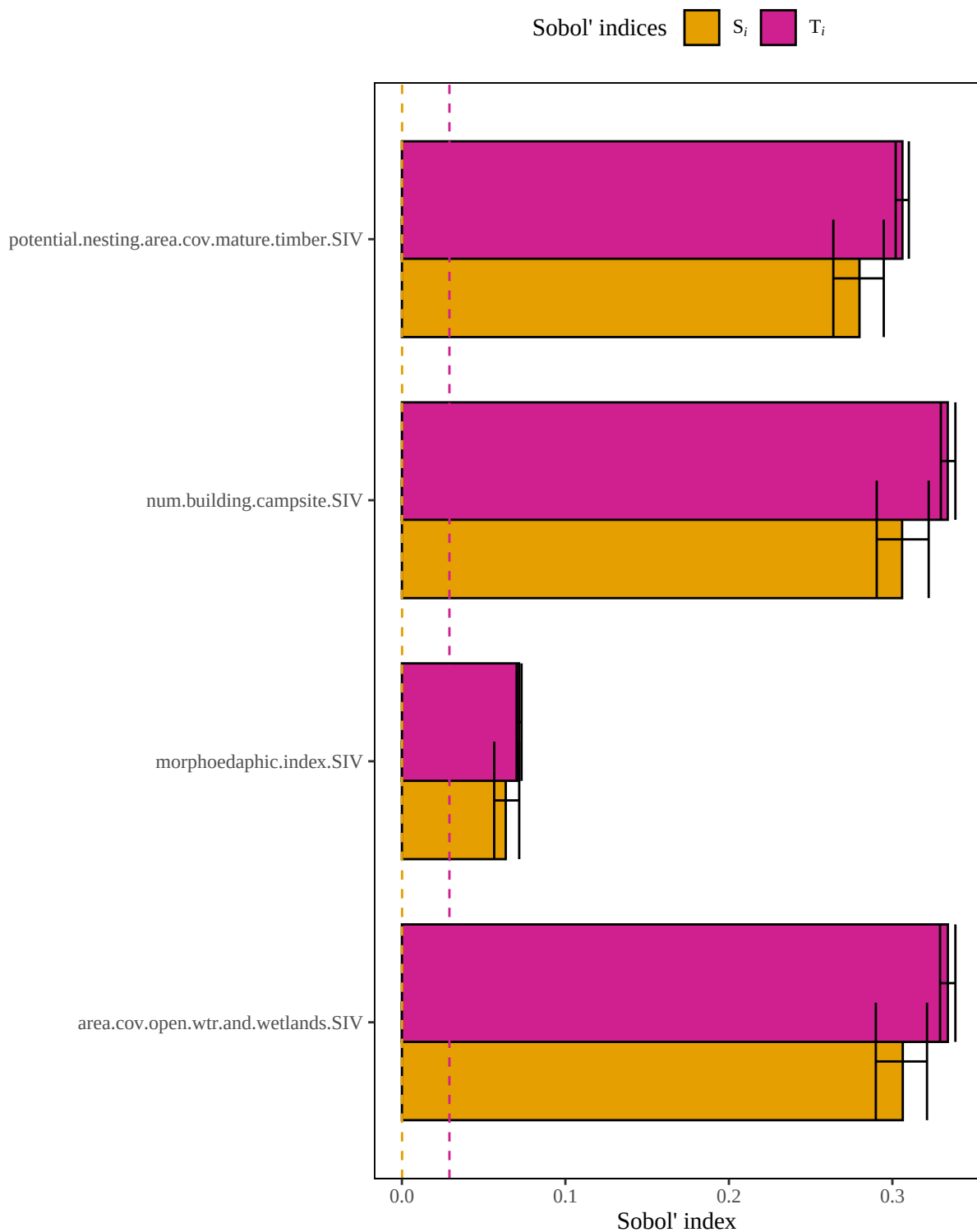
Figure 5. Results of a sensitivity analysis for the baldeagleBreeding model based on a geometric mean structure. Dashed lines represent baseline numerical approximation error for S_i and T_i ( i.e. , dummy variables).
